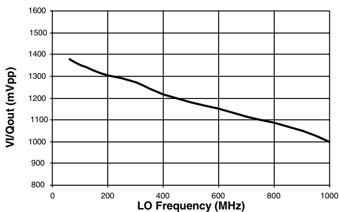
Figure 9. Typical Output Signal versus LO Frequency for P_{RF} = -15 dBm and P_{LO} = -15 dBm
